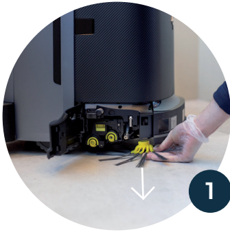
Pull to remove & clean side brush
